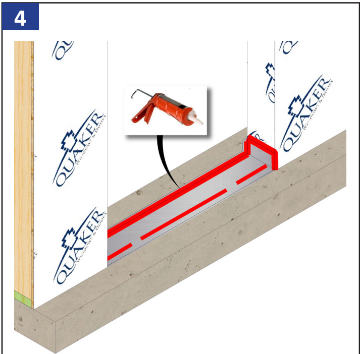
Apply a continuous bead of sealant to the exterior face of the upturned leg of the sill pan. Also seal where the pan meets the rough opening, and tool sealant over any fasteners used to install the pan. Apply a discontinuous bead of sealant across the front of the sill pan.
