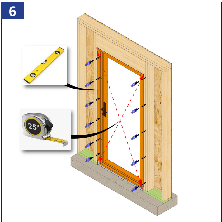
Square, level, and plumb unit in the rough opening by applying shims as needed. Do not over shim, do not shim at the head.
