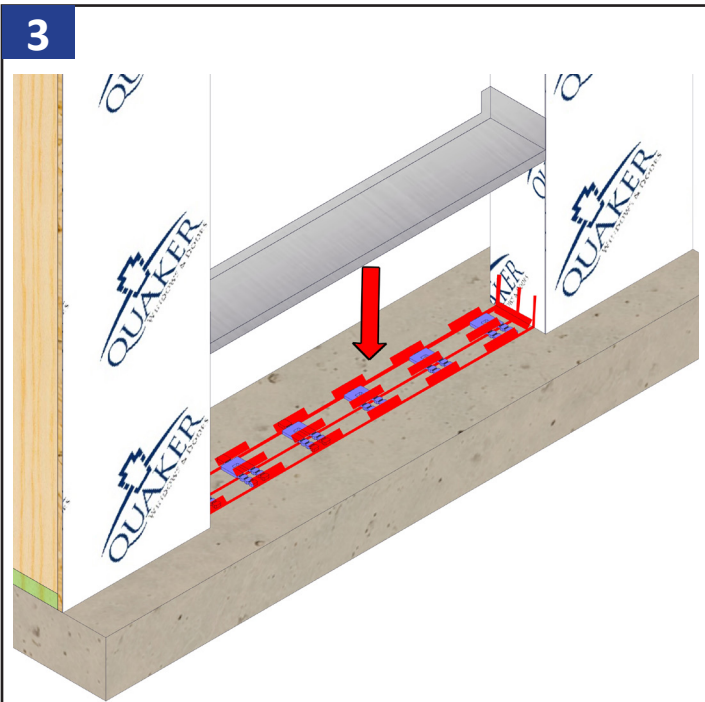
Apply sill pan flashing. The flashing must extend to the exterior face of the wall.
