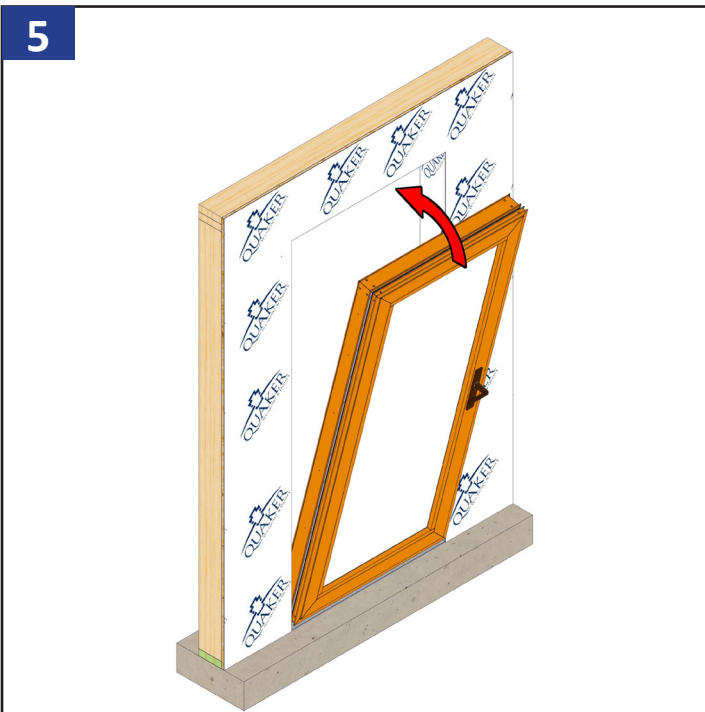
Install door by setting the bottom of the door into the rough opening and tilting into place.
